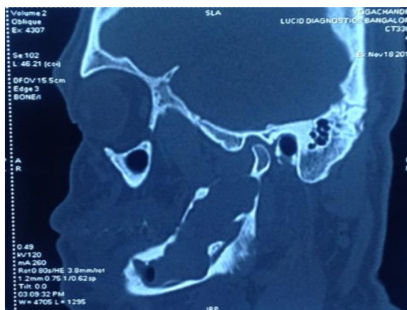
Fig. 3: (c) Sagittal section of the CT scan showing osteolytic lesion involving the body and entire ramus
